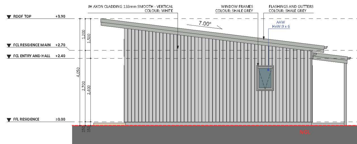
WEST ELEV. 1
