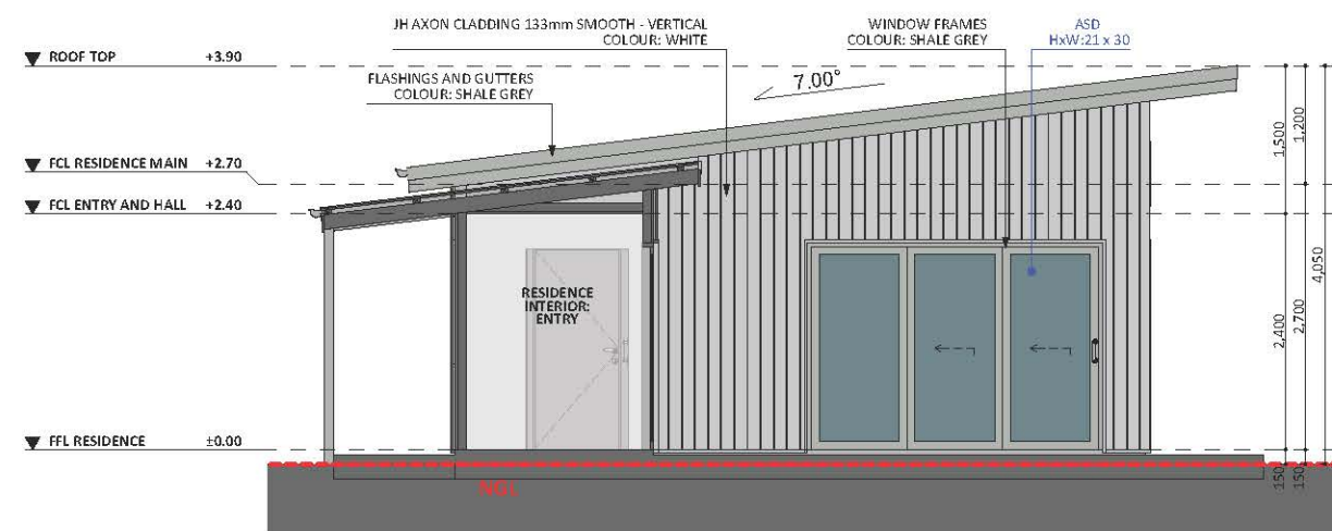
EAST ELEV. 2
