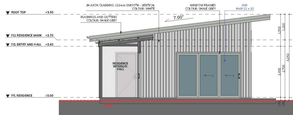
EAST ELEV. 3
