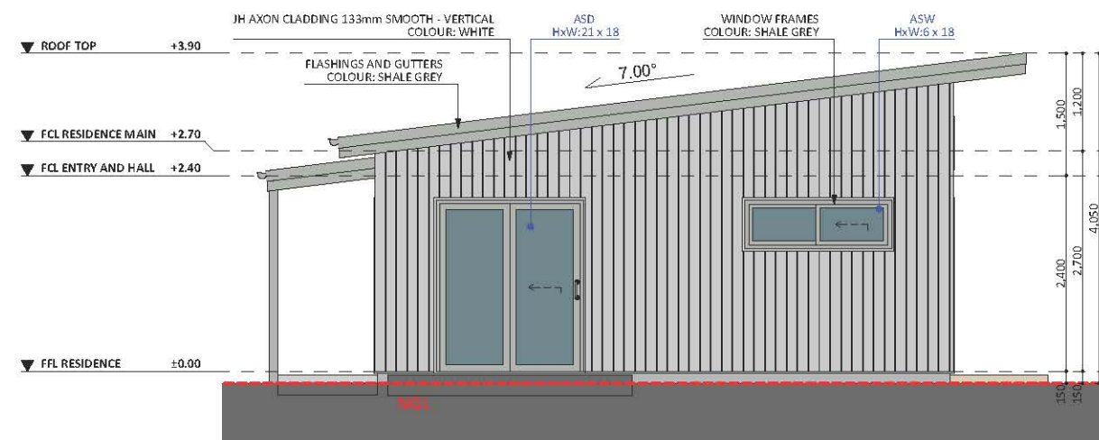
EAST ELEV. 1
