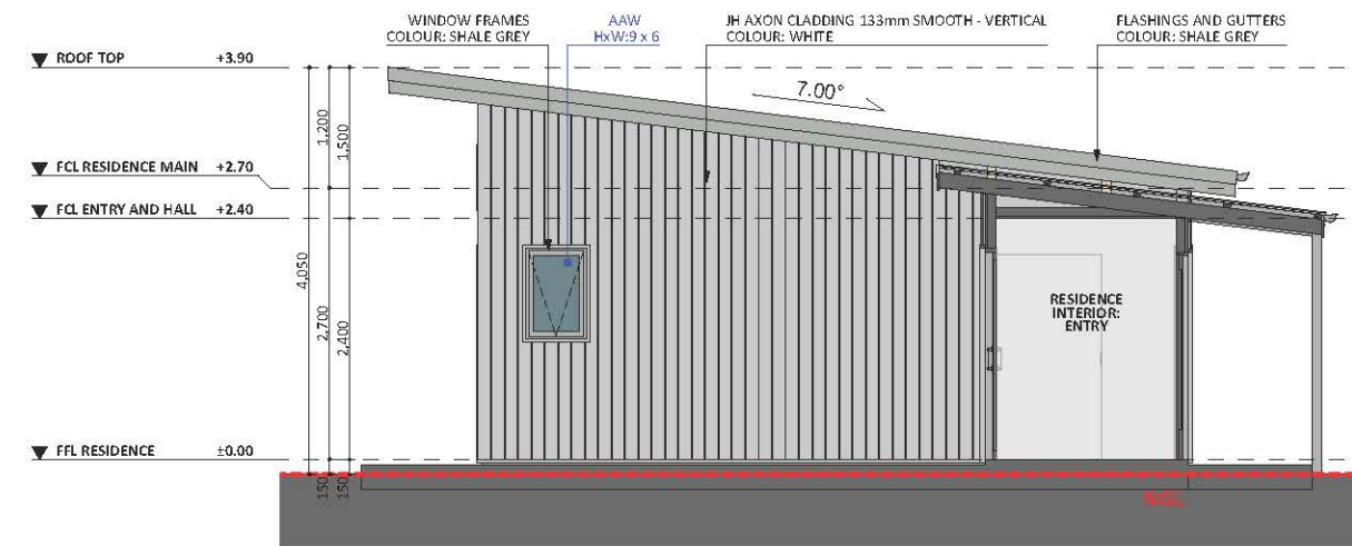
WEST ELEV. 3
