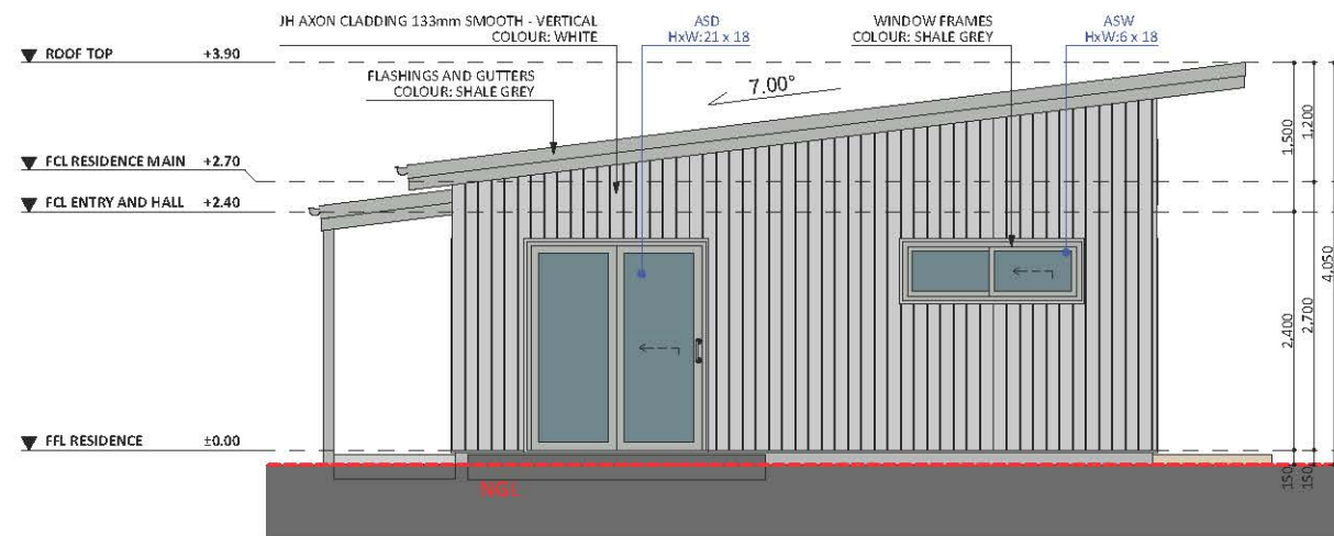
EAST ELEV. 1
