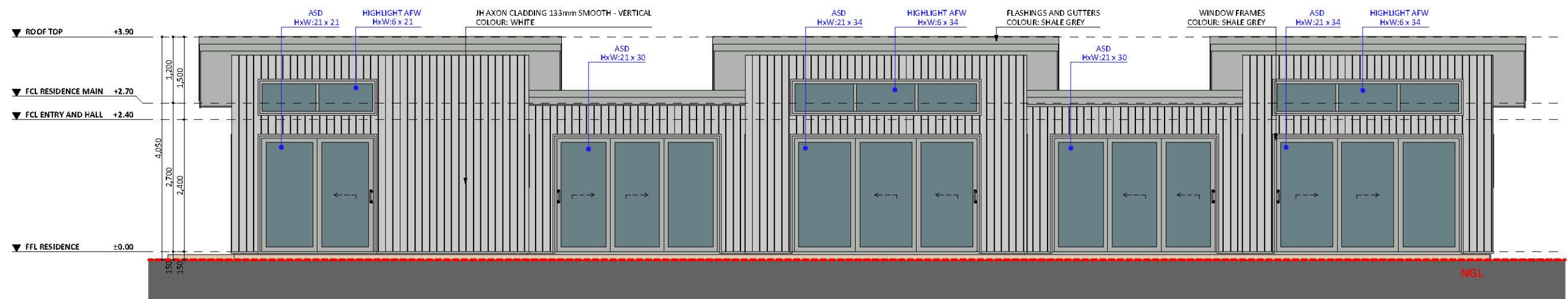
NORTH ELEV.
