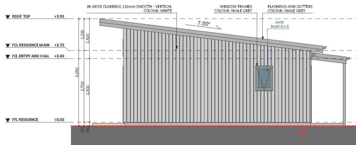
WEST ELEV. 1
