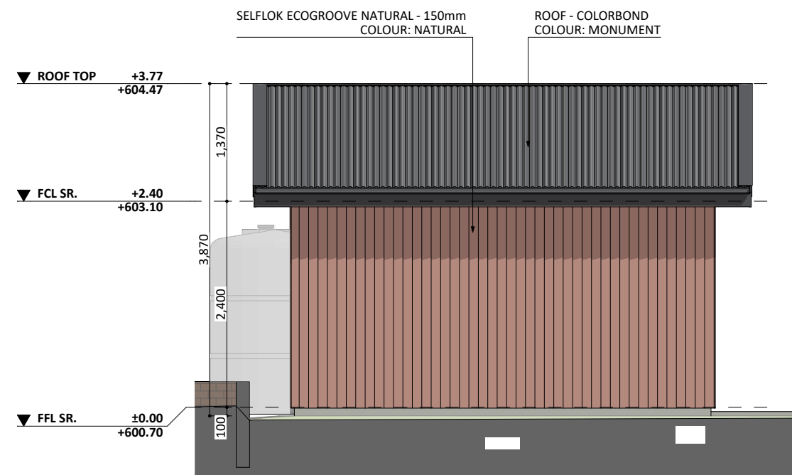
SOUTH ELEV. - SR
