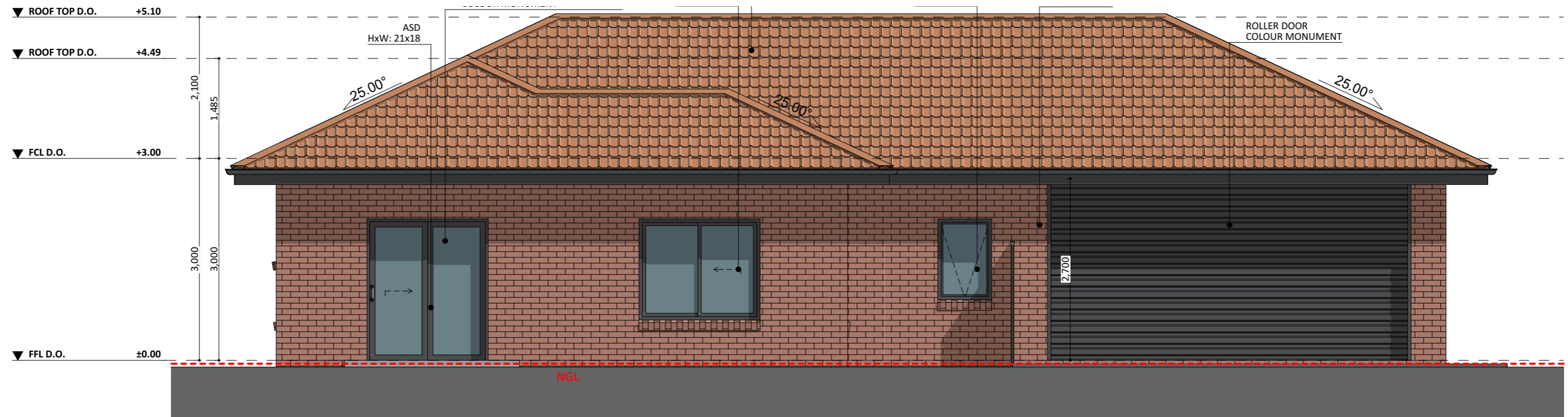
EAST ELEVATION
