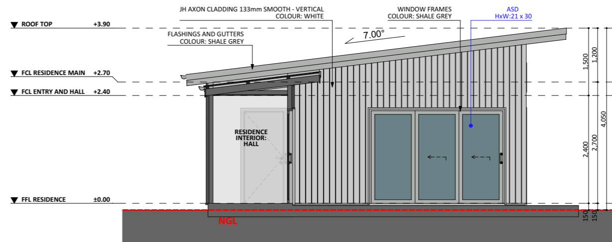
EAST ELEV. 3
