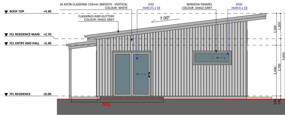
EAST ELEV. 1
