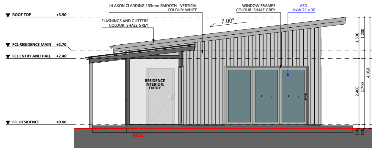
EAST ELEV. 2
