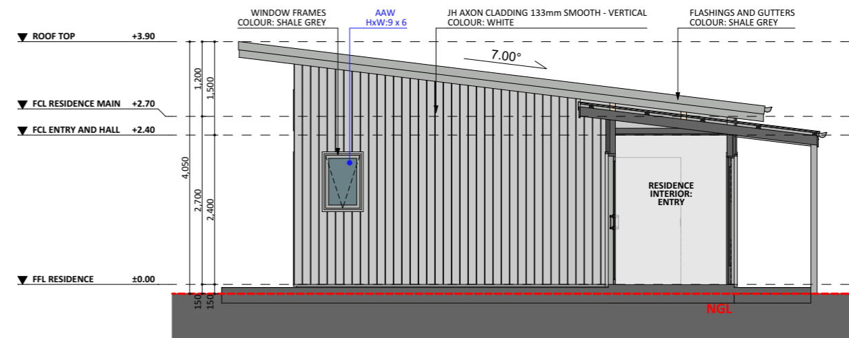
WEST ELEV. 3
