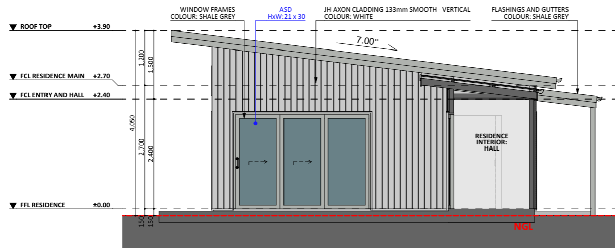
WEST ELEV. 2
