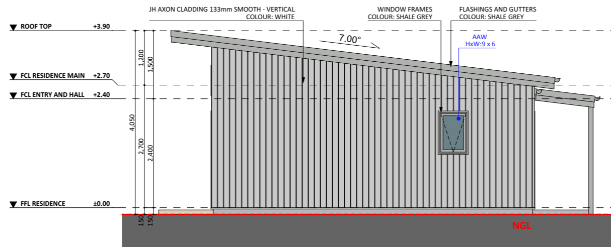
WEST ELEV. 1
